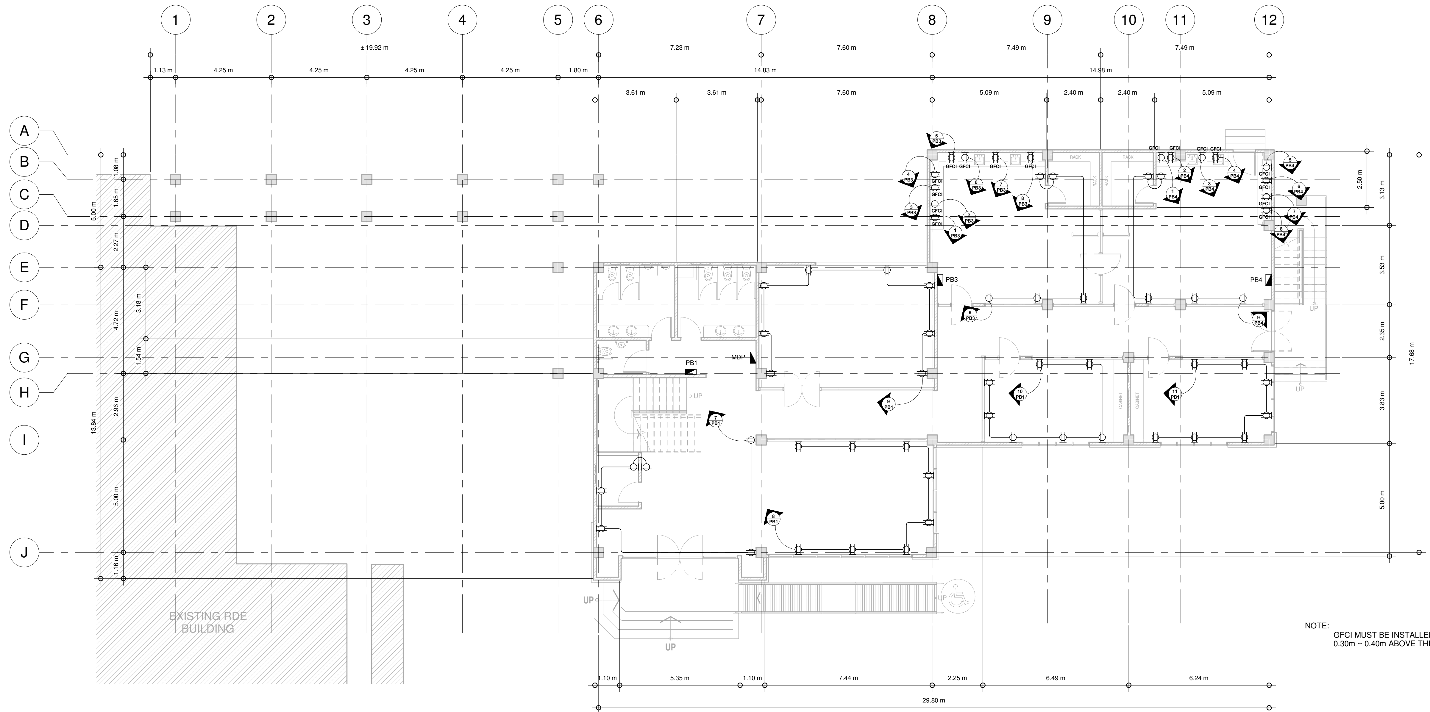
1 GROUND FLOOR CONVENIENCE OUTLET LAYOUT PLAN 1 : 100 meters
